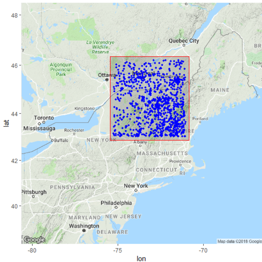
Figure 1: Global Historical Climate Network (HCN) weather stations in D3 study area.
