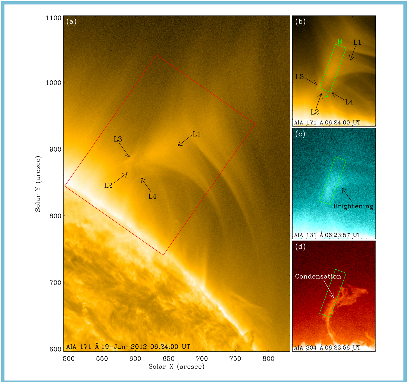
Figure 4. Figure 1 from Li et al. (2018). AIA 171Å(a,b), AIA 131Å(c), and AIA 304Å images are shown. The red rectangle in (a) shows the field of view of the other panels. An animation of panels (b-d) is available. It covers 8 hours of observing beginning at 01:00 UT on 2012 January 19. The video duration is 20 seconds.
