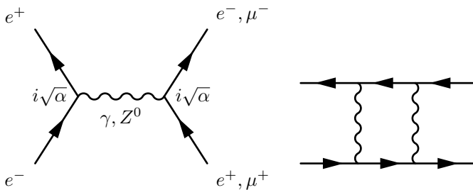
Figure 2: Using feynmp
