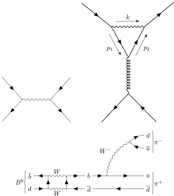
Figure 1: Using tikz-feynmann
