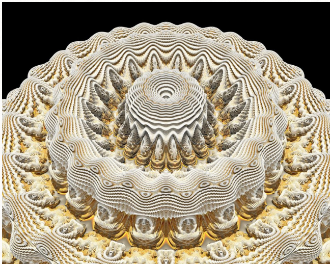
'Detail of a power 20 mandelbulb made using Visions of Chaos'. By Solerg7—Own work, Public Domain. http://bit.ly/2bcnsgM
