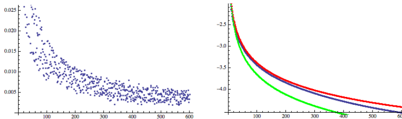
FIG. 6.5: LEFT, d(\rho_n, \psi_n, 0), 1 \leq n \leq 600 ; RIGHT, \log \frac{1}{N} \sum_{n=1}^N d(\rho_n, \psi_n, 0), 1 \leq N \leq 600 ; GREEN CURVE: -(\log N)^{.8} , RED CURVE: -(\log N)^{.85}
