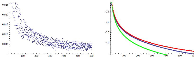
FIG. 6.5: LEFT, d(n, 1), 1 \leq n \leq 600 ; RIGHT, \log \frac{1}{N} \sum_{n=1}^N d(n, 1), 1 \leq N \leq 600 ; GREEN CURVE: -(\log N)^{.8} , RED CURVE : -(\log N)^{.85}
