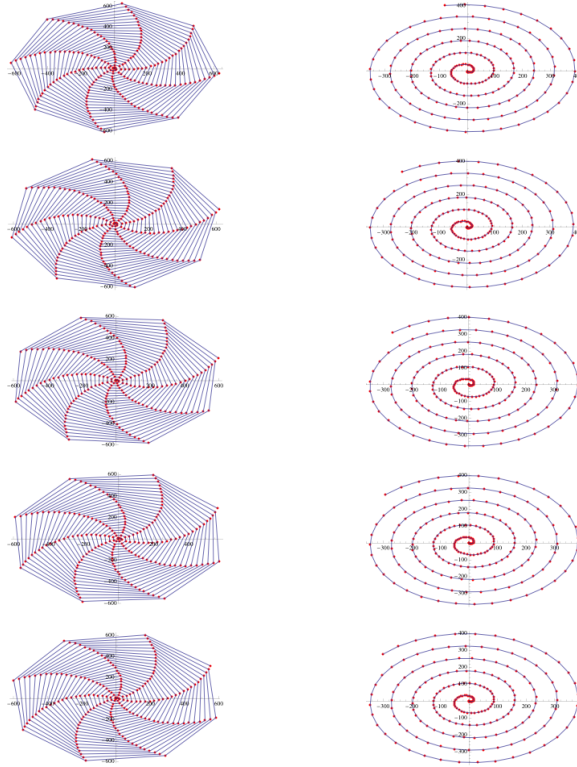
FIG. 5.2: BACKWARD ORBIT BRANCHES FOR \rho_n (1 \leq n \leq 5) CENTERED ON TWO CARDIROID ZETA FIXED POINTS
