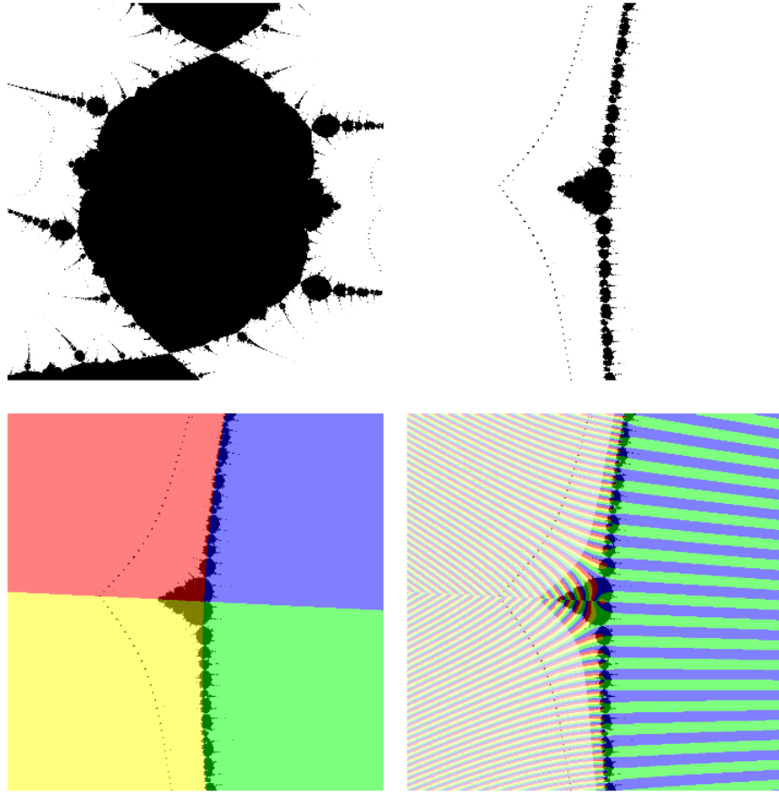
FIG. 3.5: A COPY OF A_\phi NEAR A BLUNT PROCESS OF A_\phi ; LEFT: WITH SUPERIMPOSED QUADRANT PLOT OF \zeta^{03} ; RIGHT: SUPERIMPOSED QUADRANT PLOT OF \zeta^{04}
