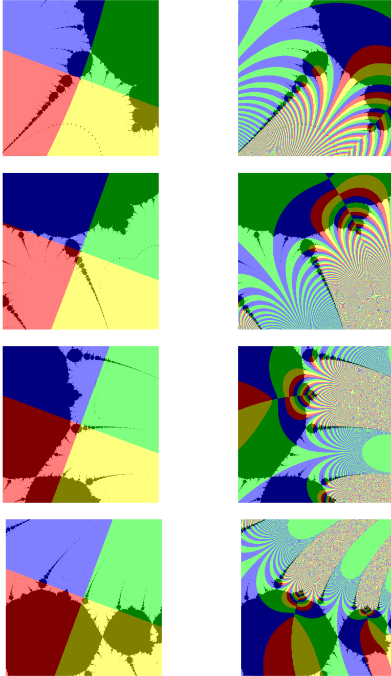
FIG. 4.1: ZOOMING IN ON \psi_{p_1} ; COLUMN 1: QUADRANT PLOTS OF \zeta(s) - s ; COLUMN 2 (TOP TO BOTTOM): QUADRANT PLOTS OF \zeta^{o_n} , n = 3, 4, 5, 6
