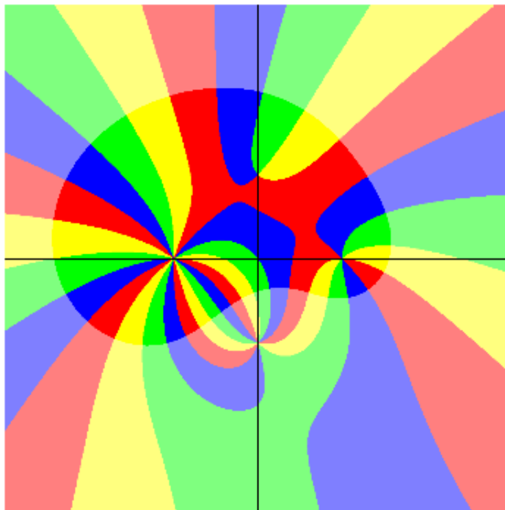
FIG. 2.1: QUADRANT PLOT OF s \mapsto (s-1)^2(s-i)(s+1)^5/(s+i)^3
