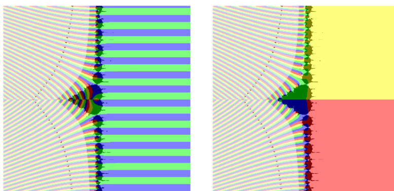
FIG. 3.2: LEFT: QUADRANT PLOT OF ZETA; RIGHT: QUADRANT PLOT OF \zeta(s) - s ; BOTH SUPERIMPOSED ON A_\phi
