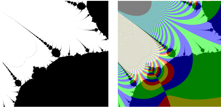
FIG. 3.1: ZEROS OF \zeta^{o2} IN FILAMENTS DECORATING THE MAIN CARDIOID
